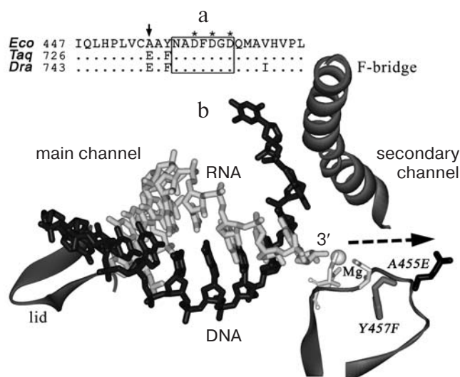
Fig. 1. Structure of the active center of RNAP. a) Alignment of RNAP \beta' -subunit sequences from E. coli (Eco), T. aquaticus (Taq), and D. radiodurans (Dra) in the area of the NADFDGD-motif. Numbers correspond to the amino acid residues at the left alignment border; asterisks denote the aspartic acid residues involved in magnesium ion binding; the arrow points to the A455 residue. b) A model of nucleic acid localization in the elongation complex of T. thermophilus RNAP (from data of [10]). The figure displays the main and secondary RNAP channels, RNA is drawn in light-gray, template DNA in black. An area of the \beta' -subunit containing the NADFDGD-motif (amino acids 447–472, numbering of E. coli ) is in the bottom right hand corner of the figure. A gray sphere denotes the magnesium ion bound in the active center; three aspartic acid residues of the NADFDGD-motif are drawn in light gray. The amino acid substitution A455E is drawn in black, the substitution Y457F in gray. Arrow points to a pathway of the RNA 3'-end movement upon a backtracking of the elongation complex. In addition, two elements of \beta' -subunit are drawn between which the RNA–DNA hybrid is positioned: the “lid” located at the rear of the hybrid and the “F-bridge” separating the main and the secondary channels.
